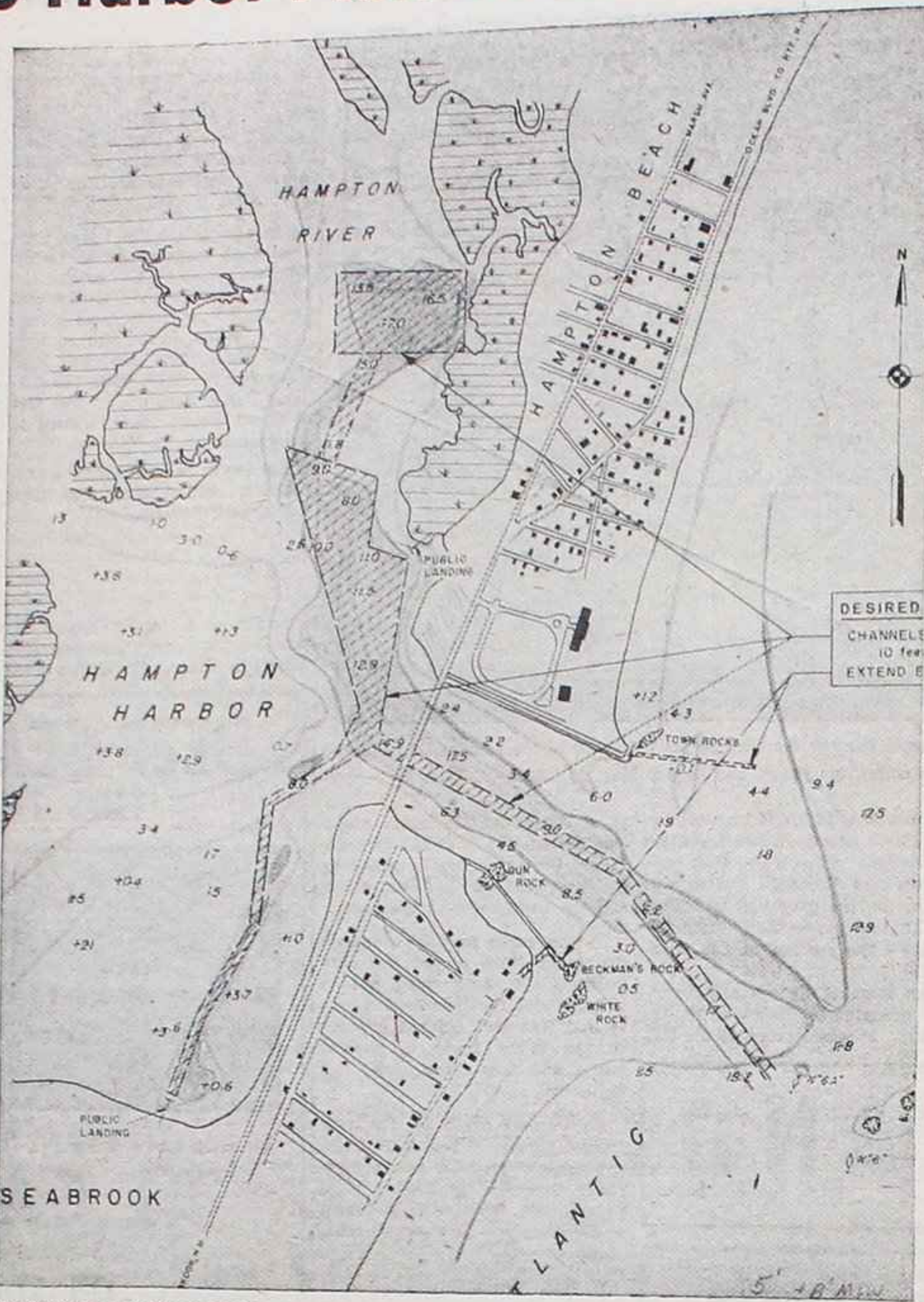
PROPOSED IMPROVEMENTS for Hampton Harbor inlet estimated to cost $365,000 were submitted this week by Army Engineers in a report to the N. H. Port Authority. Plans call for the extension of the north and south jetties and the digging of a new channel 8 feet deep by 150 feet wide at the entrance to the harbor.
